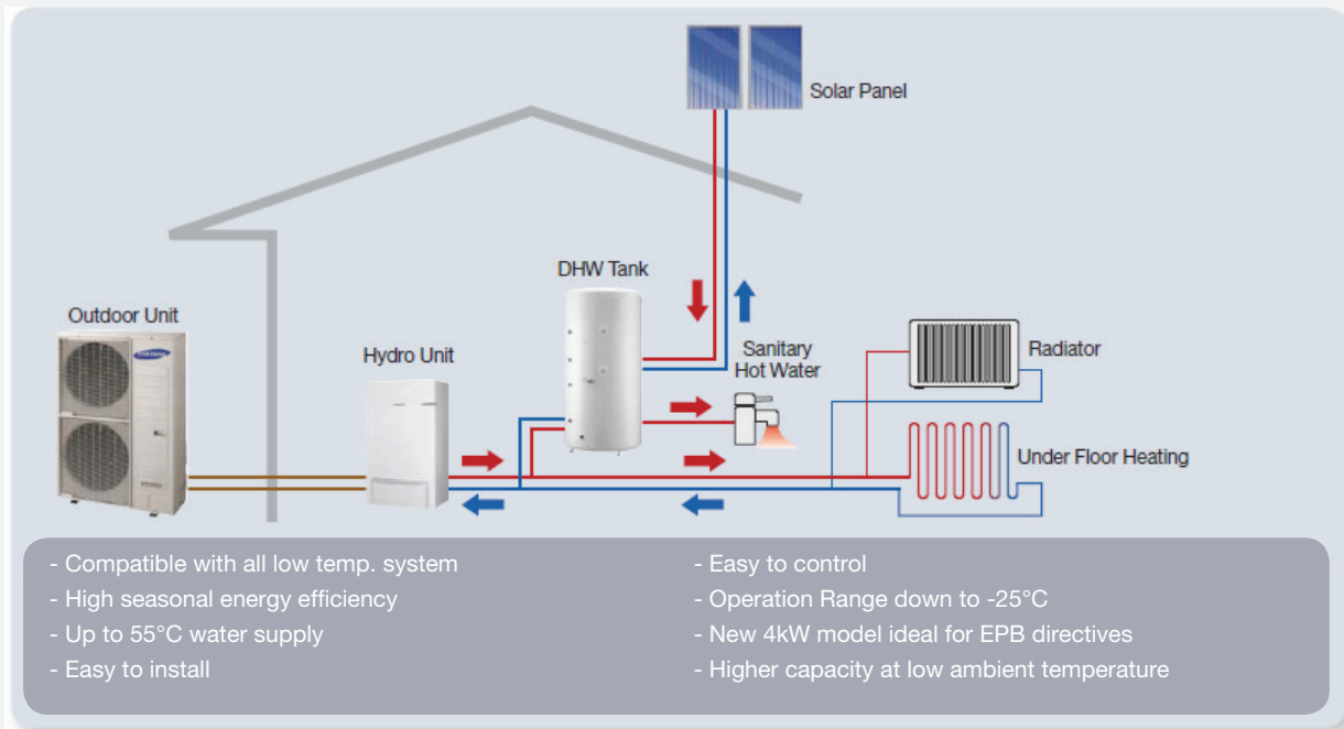
EHS Split process overview (air-to-water)
