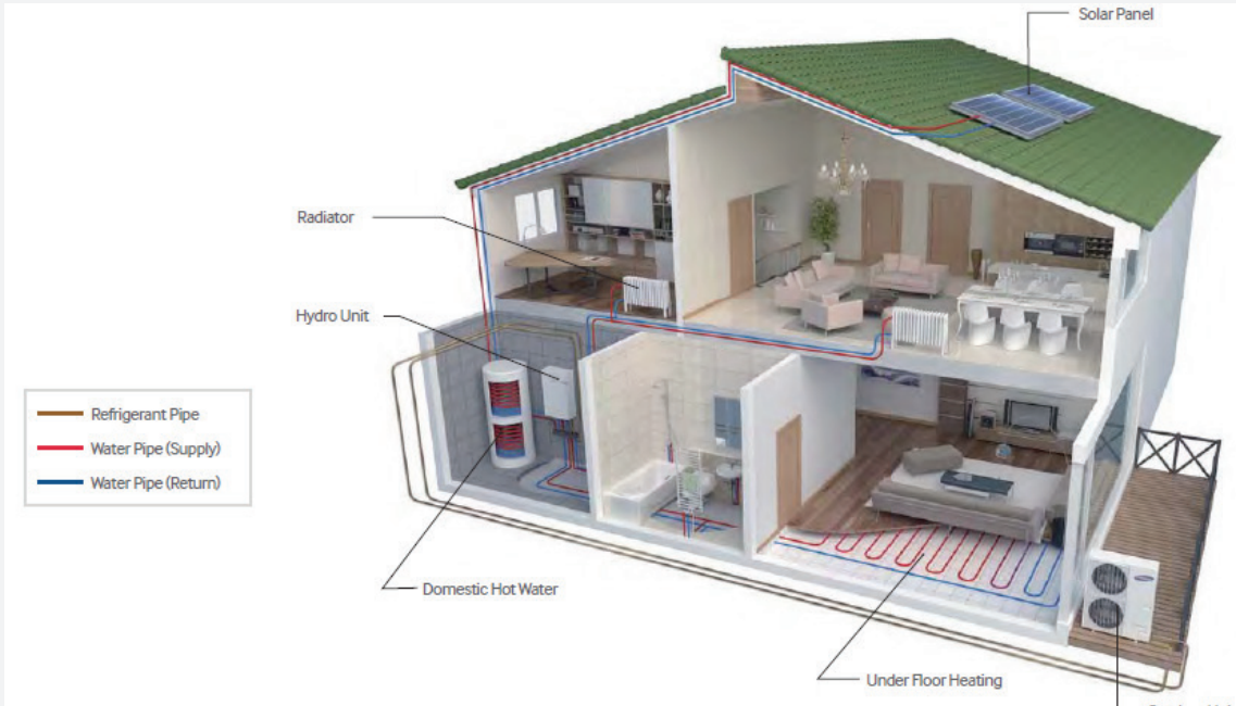
EHS Split process overview (air-to-water)
