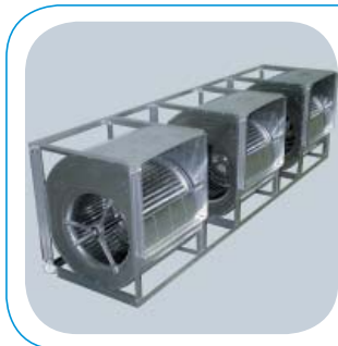
CBP-TC Double inlet triplex centrifugal fans
